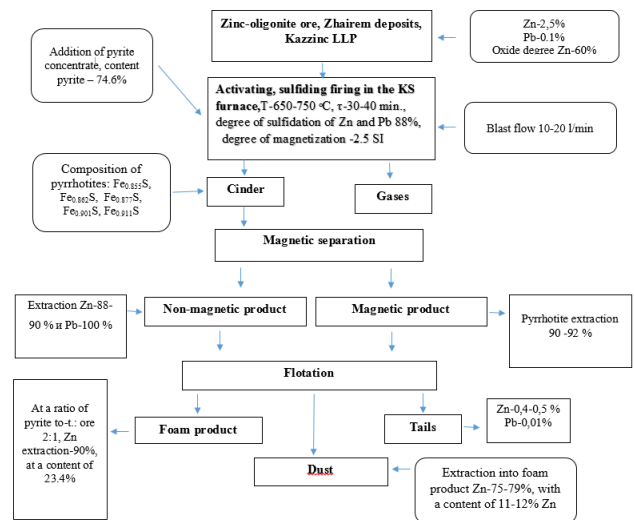
Figure 5 - Flow diagram of the technology for high-temperature sulfiding roasting of oxidized lead-zinc ore in a fluidized bed furnace
