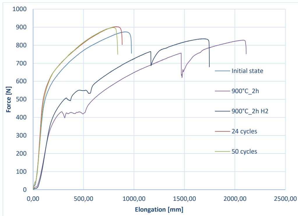
Fig. 5 - Tensile curves for delivery state and after hydrogenation proces
