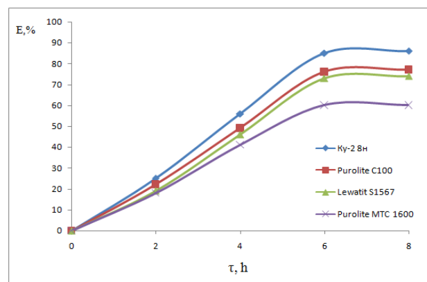
Figure 1-Lanthanum sorption from model solutions
