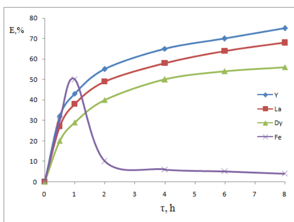
Figure 2- Sorption of rare-earth elements and iron from model solutions
