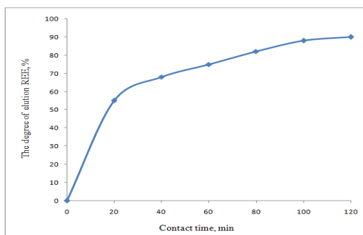
Figure 4 – Change in the degree of elution of lanthanum from the phase of cation exchanger KU-2-8-n in time
