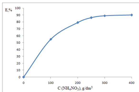
Figure 3 - Dependence of changes in the degree of elution of lanthanum on the concentration of ammonium nitrate
