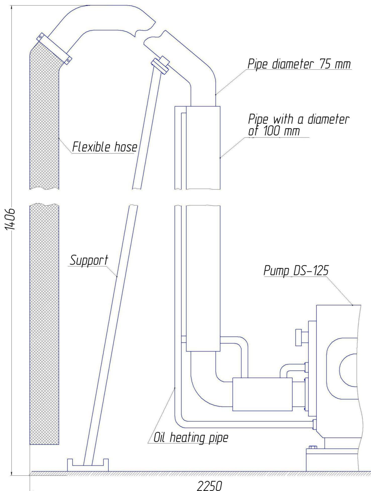
Figure 4 – Bitumen loading device
