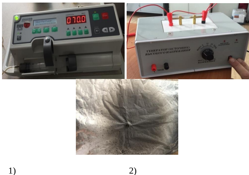
Figure 2 - Laboratory installation of electrospinnagug: pump syringe (1), high-voltage power source (2), substrate of aluminum foil (3)
