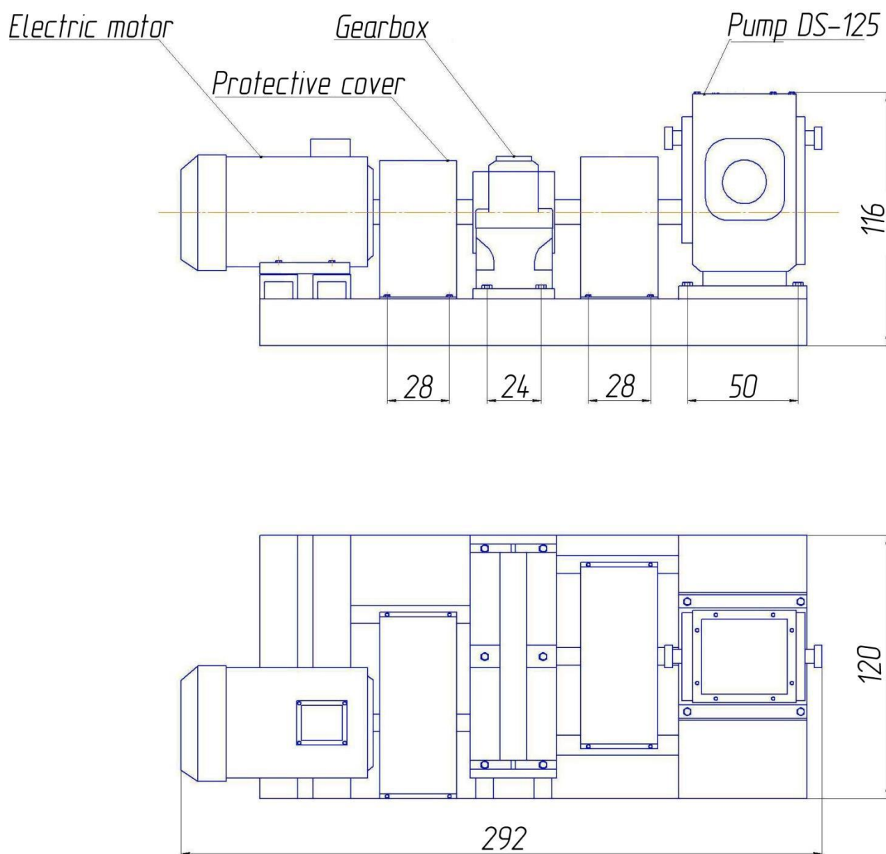
Figure 3 – Installation of bitumen pumping
