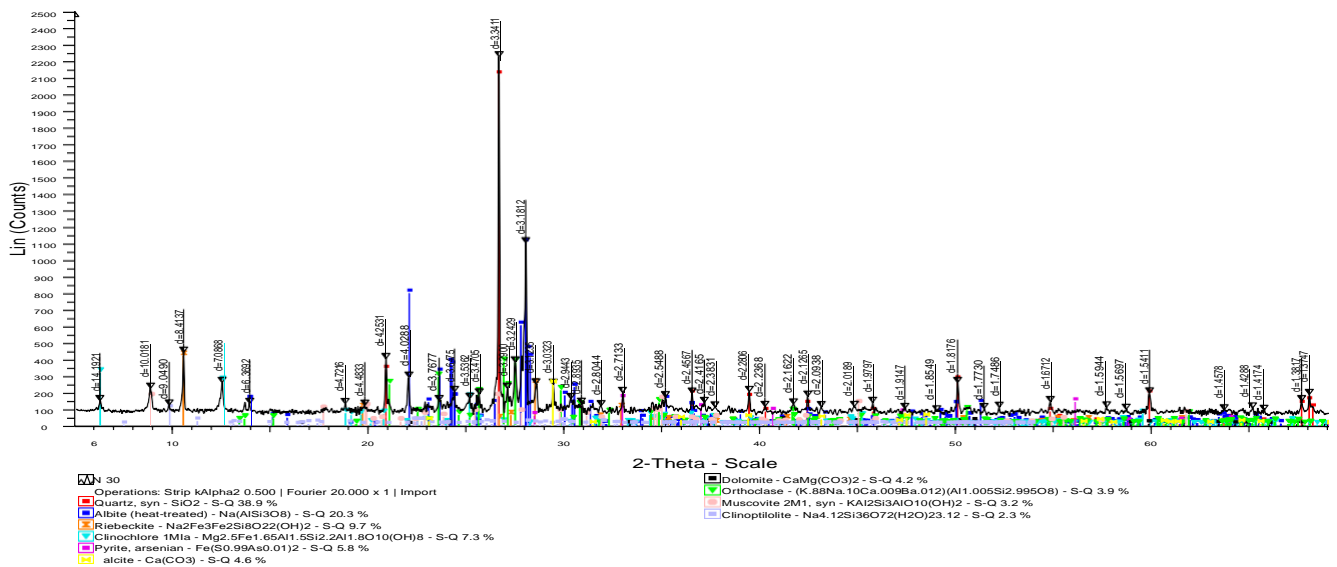
Figure 1 - The results of x-ray phase analysis of ore samples
