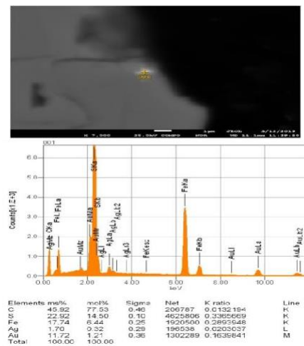
Figure 2 - Electron-microscopic analysis of ore
